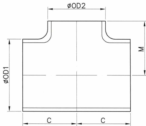
REDUCING TEE
