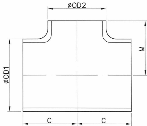
REDUCING TEE
