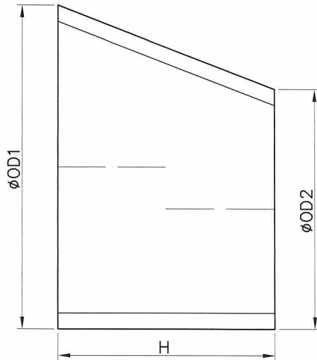
ECC. REDUCER
