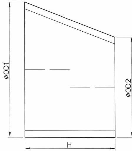
ECC. REDUCER
